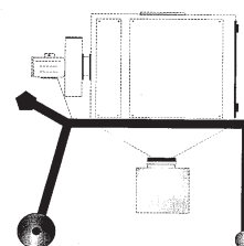
SV-1100 WITH A HOPPER AND MOBILE CART
