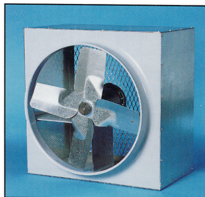
Fan shown c/w Rear Sleeve and Back Guard (Front View)
