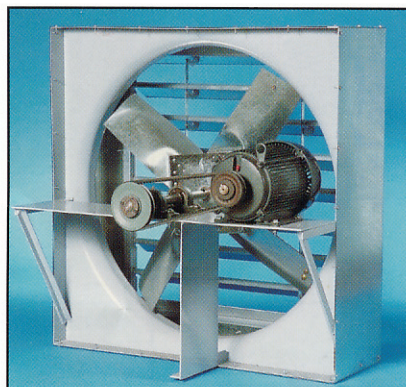
Fan shown c/w Front Sleeve and Shutter (Rear View)
